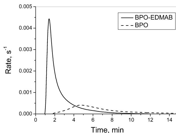
Figure 13. Polymerization rate vs time of Bis-phenol-A-bis(glycidyl methacrylate) at 80 °C using as initiator either the redox system benzoyl peroxide/ethyl 4-(dimethylamino)benzoate or benzoyl peroxide alone.
