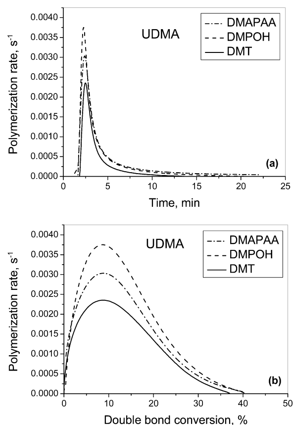
Figure 5. Effect of the amine chemical structure on the profile of the polymerization rate vs time (a) or double-bond conversion (b) for the urethane dimethacrylate (UDMA) polymerization at 37 °C, initiated by the benzoyl peroxide (BPO)/amine system. [BPO] = [amine] = 0.5 mol %.
