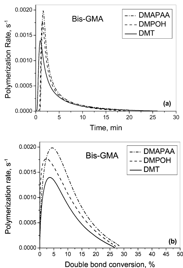
Figure 4. Effect of the amine chemical structure on the profile of the polymerization rate vs time (a) or double-bond conversion (b) for the Bis-phenol-A-bis(glycidyl methacrylate) (Bis-GMA) polymerization at 37 °C, initiated by the benzoyl peroxide (BPO)/amine system. [BPO] = [amine] = 0.5 mol %.
